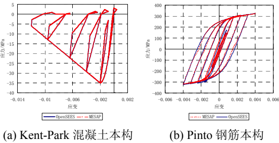
图 11 材料模型滞回曲线 Fig.11 Hysteretic curve of the material model
