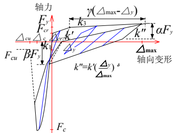
图 6 Fishinger 弹簧本构 Fig.6 Fishinger spring model
