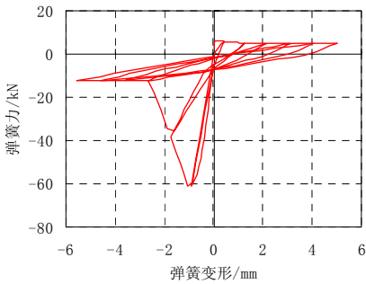
图 12 Fischinger 轴向弹簧本构滞回曲线 Fig.12 Hysteretic curve of Fischinger spring model
