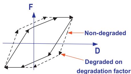
Figure 8. Hysteretic loop of energy degradation
